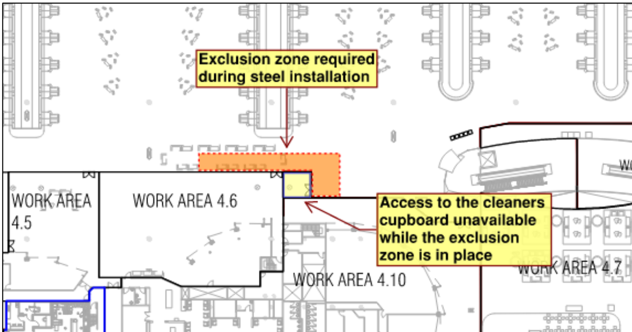
Figure 1: Exclusion Zone – Structural Steel Installation
