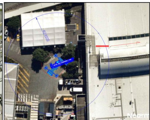
Figure 3: Temporary Laydown and Crane Lifting
